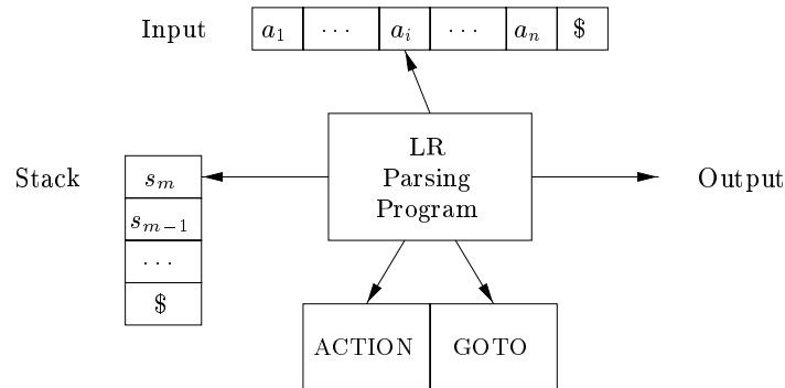
Figure 4.35: Model of an LR parser
