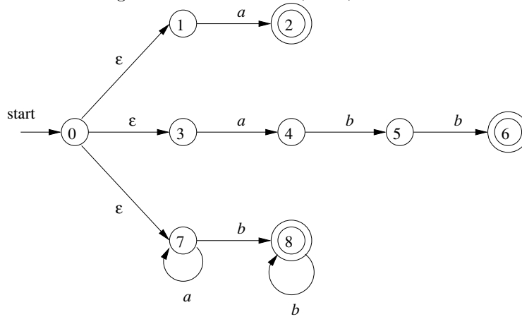
Figure 3.52: Combined NFA
