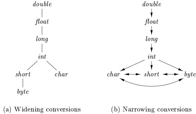
Figure 6.25: Conversions between primitive types in Java
