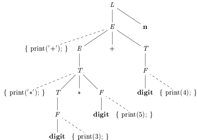
Figure 5.22: Parse tree with actions embedded
