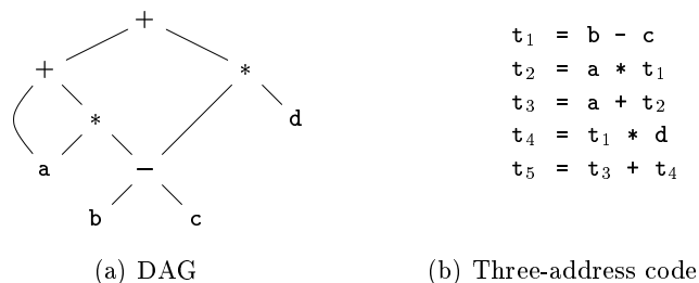
Figure 6.8: A DAG and its corresponding three-address code
