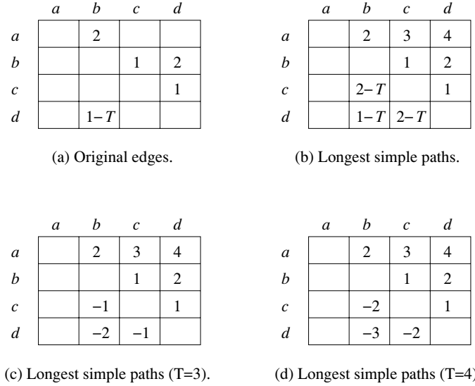
Figure 10.28: Transitive dependences in Example 10.20
