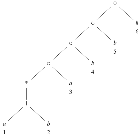
Figure 3.56: Syntax tree for (a|b)^*abb\#
