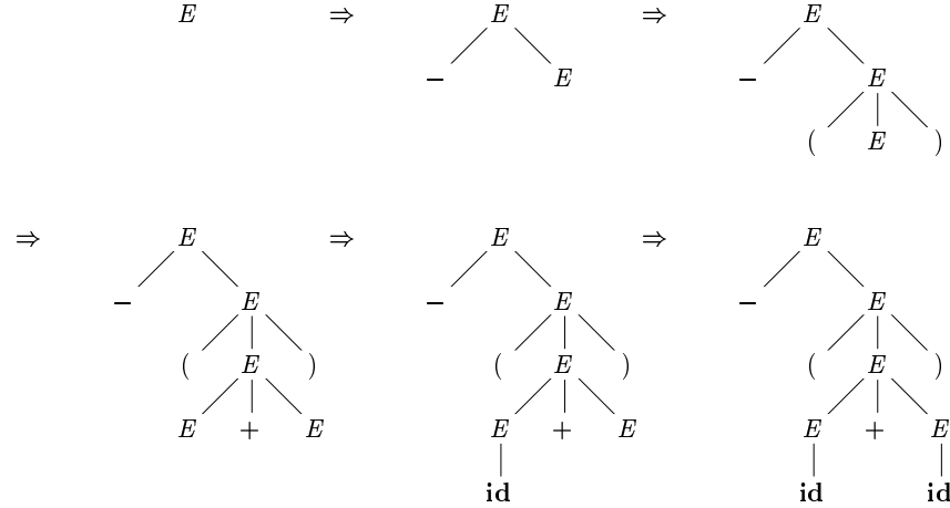
Figure 4.4: Sequence of parse trees for derivation (4.8)
