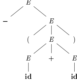
Figure 4.3: Parse tree for -(\text{id} + \text{id})
