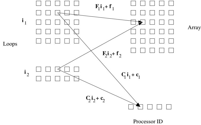
Figure 11.25: Space-partition constraints
