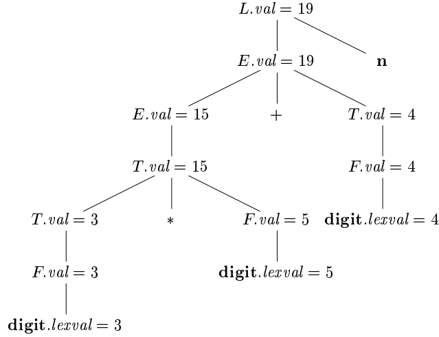
Figure 5.3: Annotated parse tree for 3 * 5 + 4 \mathbf{n}
