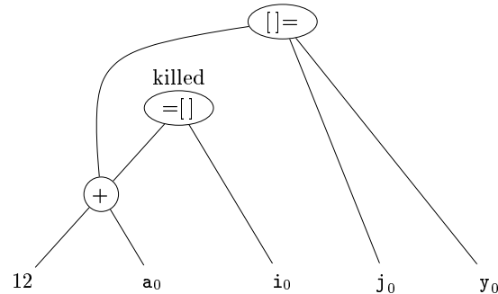
Figure 8.15: A node that kills a use of an array need not have that array as a child
